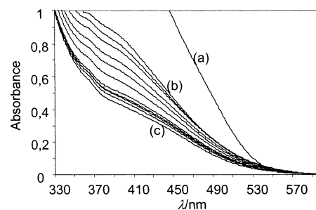
Figure 5. UV–visible study of the interaction between \text{Cp}^*\text{Fe}(\text{dppe})\text{H} and HFIP (5 equiv) in \text{CH}_2\text{Cl}_2 . [\text{Fe}] = 0.02 M. (a) Before the HFIP addition. (b) T = 270 K. (c) T = 200 K. The other intermediate spectra correspond to 265–225 K (5 K steps).
